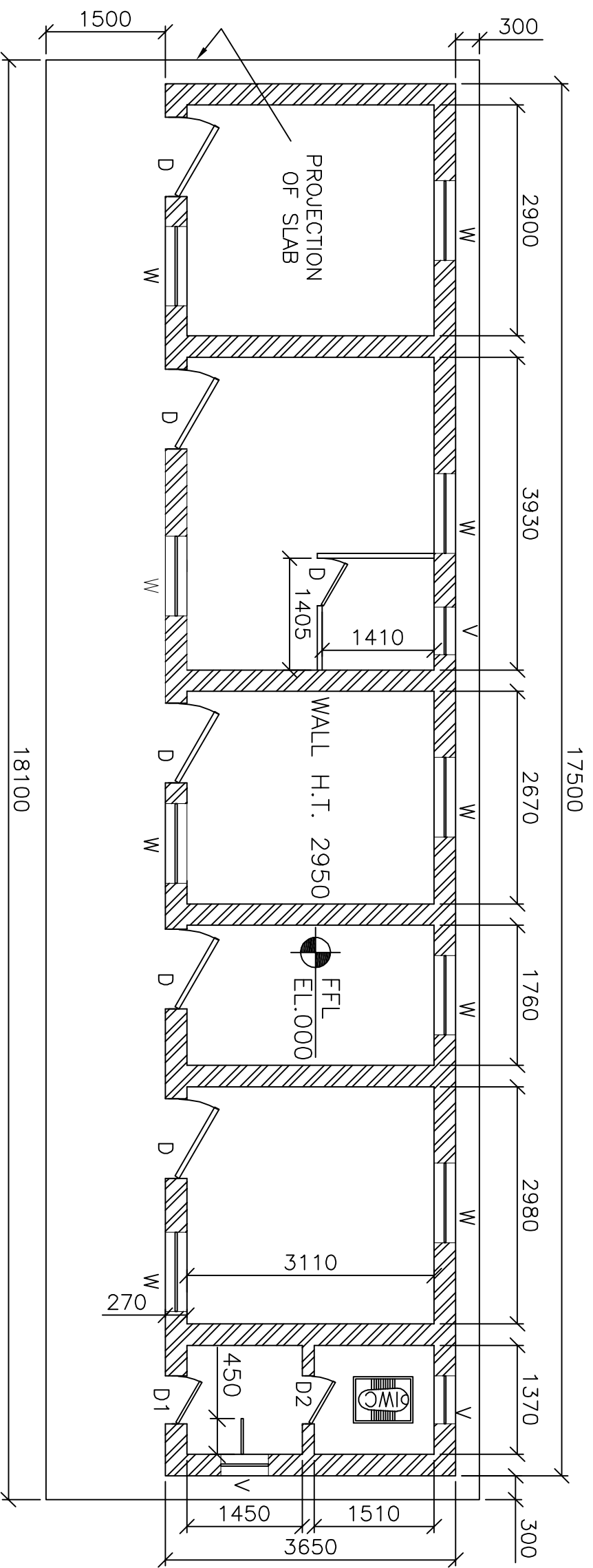
LAYOUT OF CISF GATE OFFICE (SCALE 1:75)
