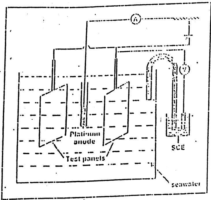
Figure 1 : Diagrammatic sketch of the apparatus for determining resistance to seawater under conditions of cathodic protection.
