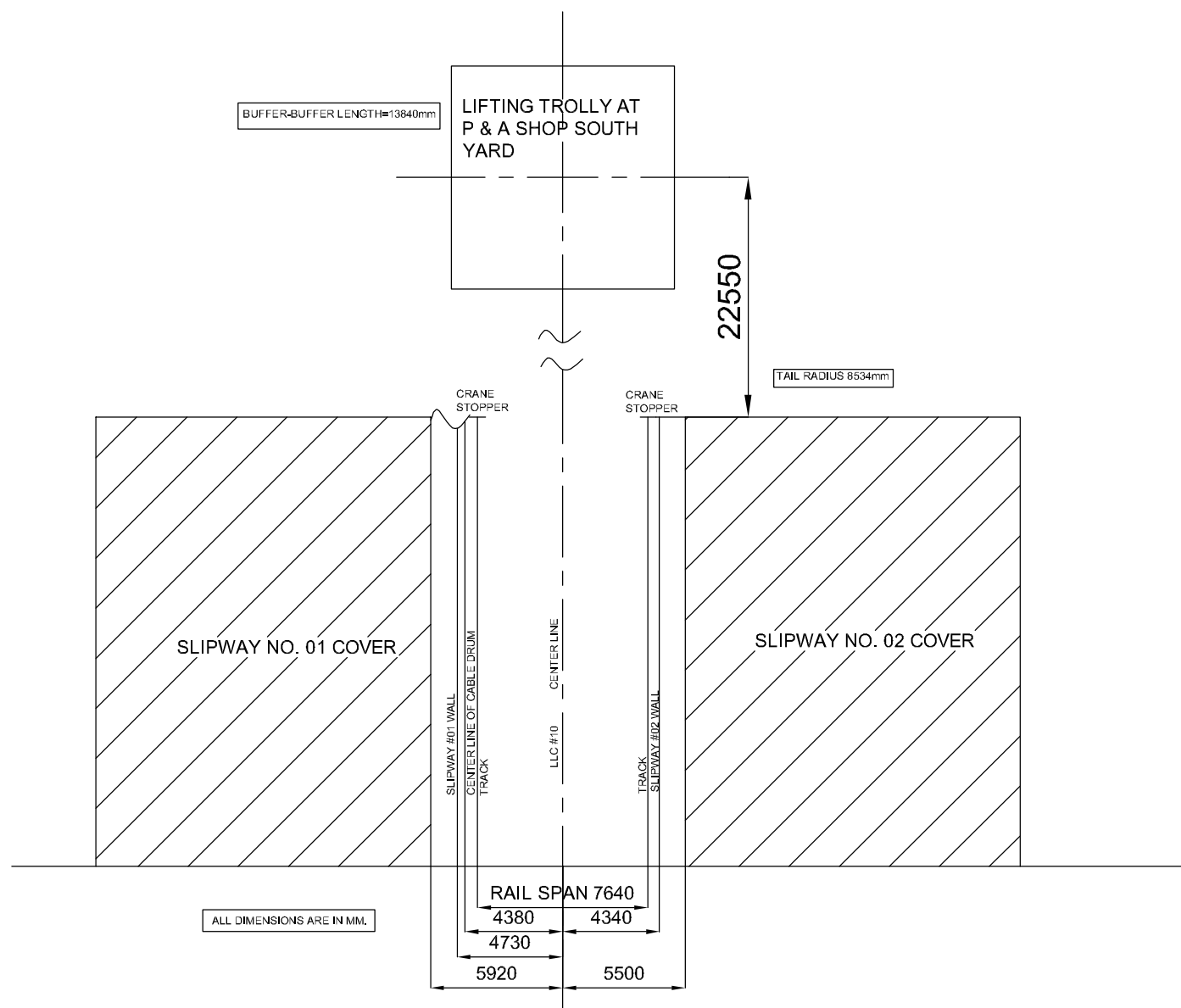
PLAN VIEW OF LL CRANE #10
