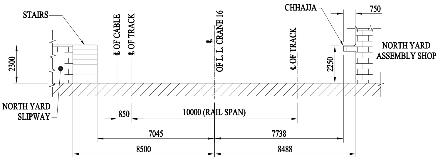
ENLARGED VIEW AT THE STAIRCASE OF SLIPWAY
