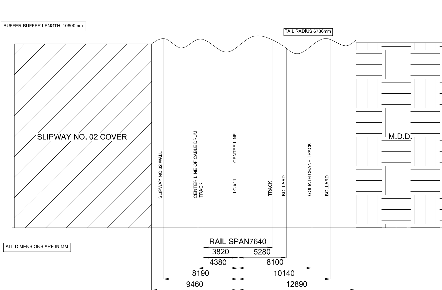
PLAN VIEW OF LL CRANE #11
