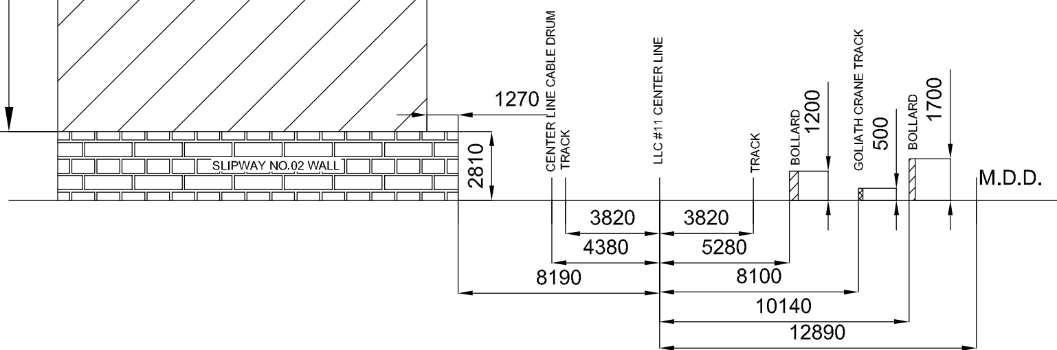
ELEVATION VIEW OF LL CRANE #11
