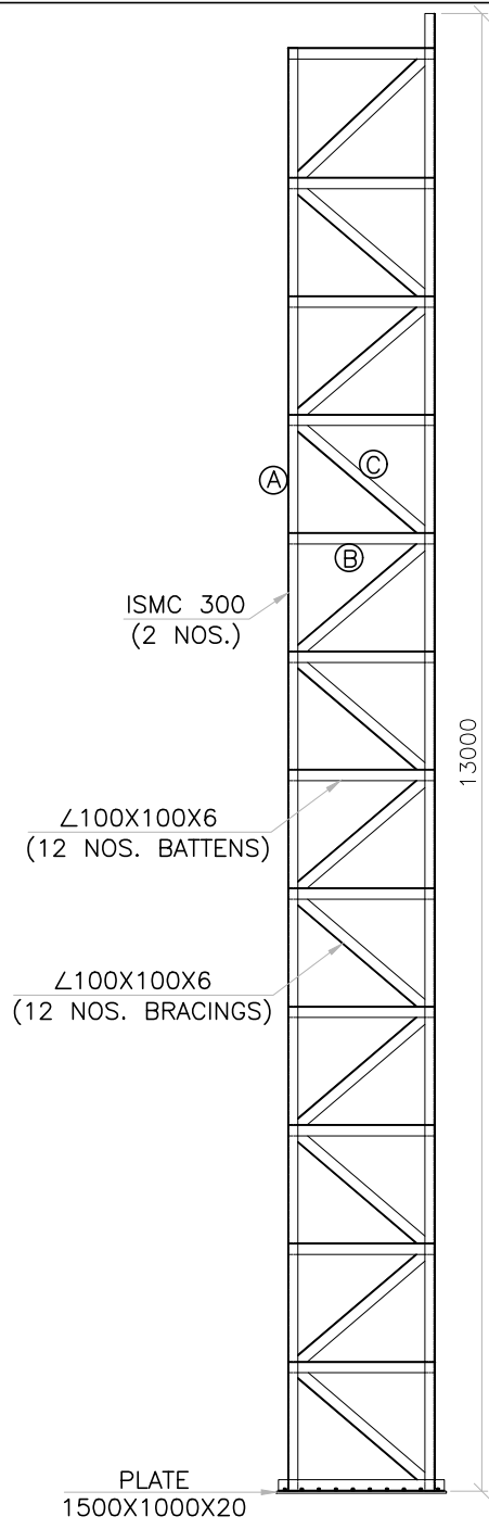
FRONT ELEVATION
