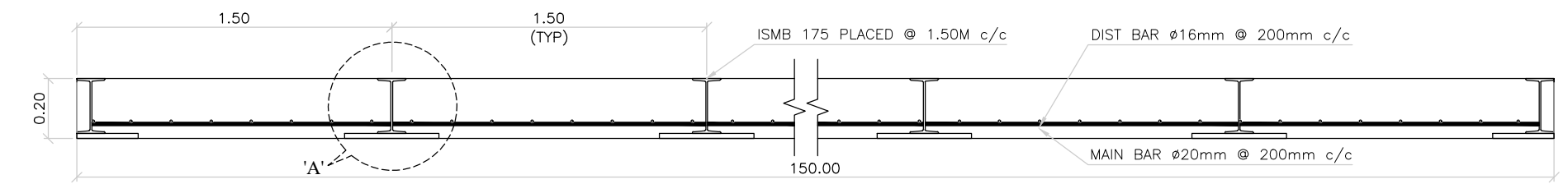
SECTION 1-1
