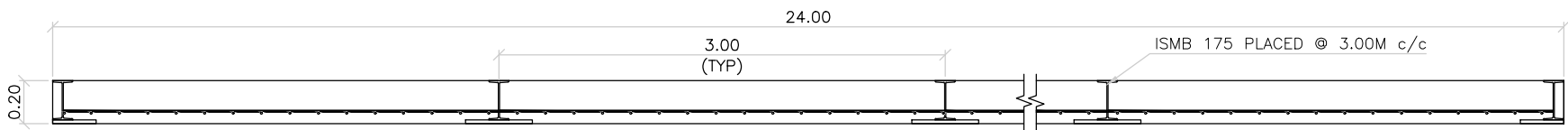
SECTION 2-2
